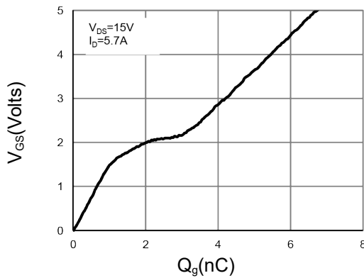
Figure 7: Gate-Charge Characteristics
