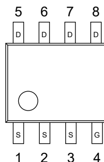
SOP-8
