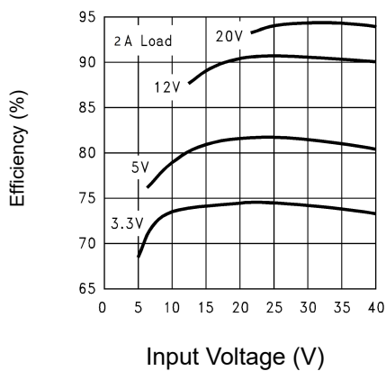
Figure 3: Efficiency
