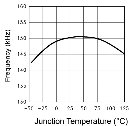
Figure 12: Switching Frequency
