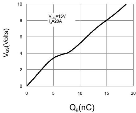
Figure 7: Gate-Charge Characteristics
