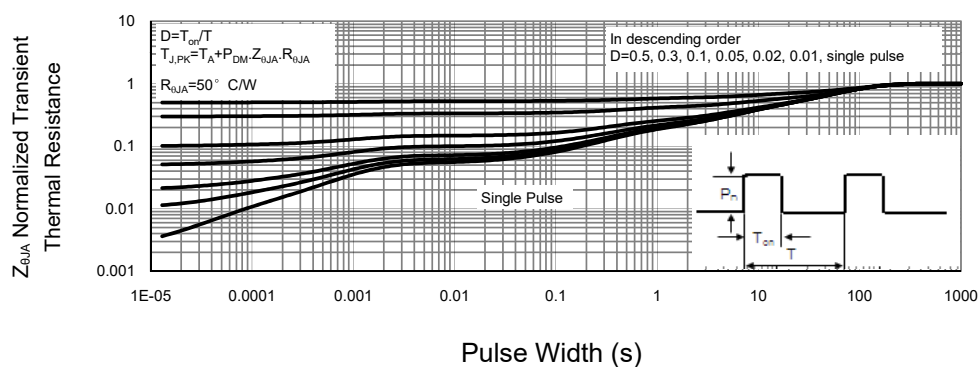
Figure 15: Normalized Maximum Transient Thermal Impedance (Note H)
