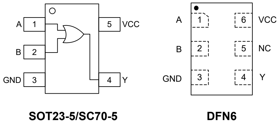
Figure1. Top View
