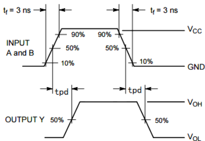
Figure 3. Switch Waveform
