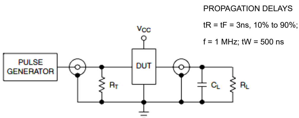
Figure4. Test Circuit
