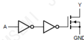
Figure 3. Logic diagram
