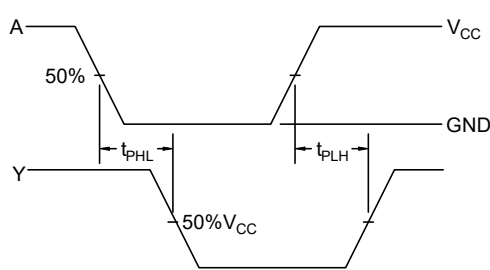
Figure3. Switching Waveform
