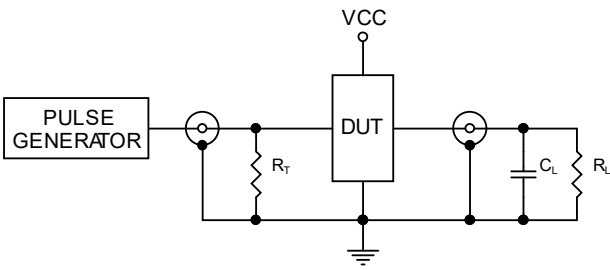
Figure4. Test Circuit
