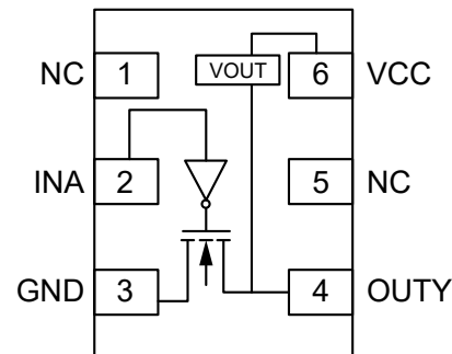
DFN6
