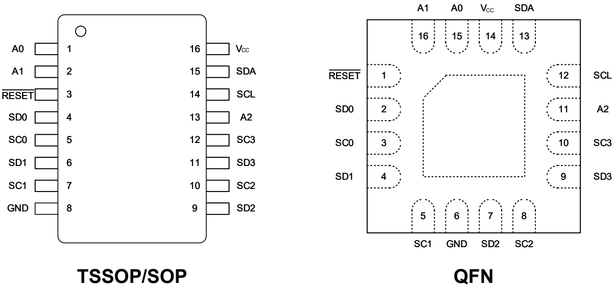
Pin Functions of Package TSSOP/SOP
