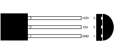
TO-92
