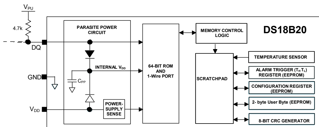
Figure 1. DS18B20 Block Diagram
