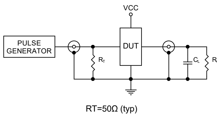
Figure4. Test Circuit
