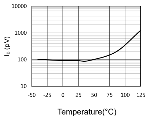
Figure 8: Input Bias vs Temperature
