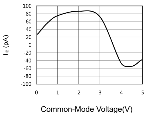
Figure 7: IB vs Common-mode Voltage
