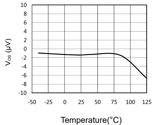
Figure 2: Offset Voltage vs Temperature
