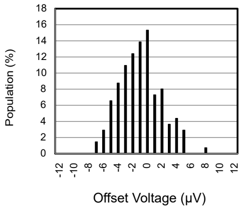
Figure 1: Offset Voltage Distribution
