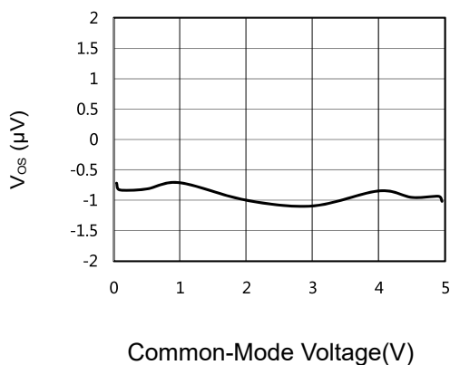
Figure 9: Vos vs Common-mode Voltage
