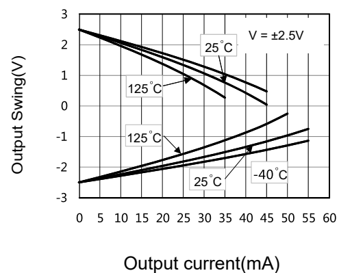
Figure 6: Output Swing vs Load Current
