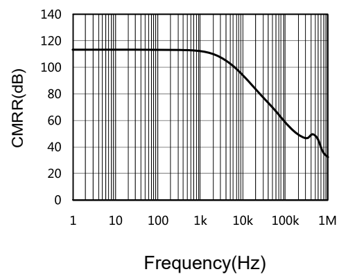
Figure 4: CMRR vs Frequency
