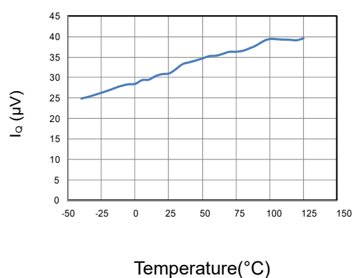
Figure 10: Quiescent Current vs Temperature
