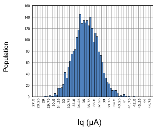
Figure 11: Quiescent Current Distribution
