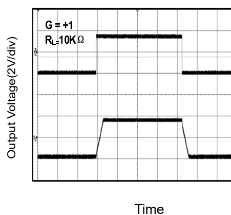
Figure 12: Large-Scale Step Response
