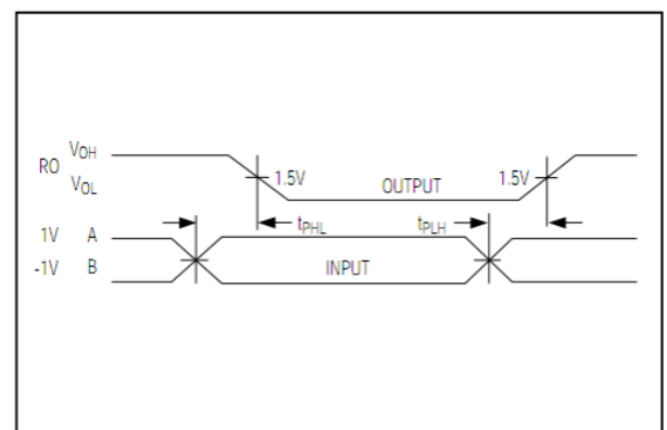
Figure13 RecelverPropagationDelaySequence
