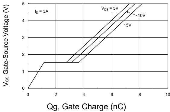
Figure 7: Gate-Charge Characteristics
