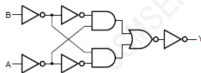
Figure 3. Logic diagram
