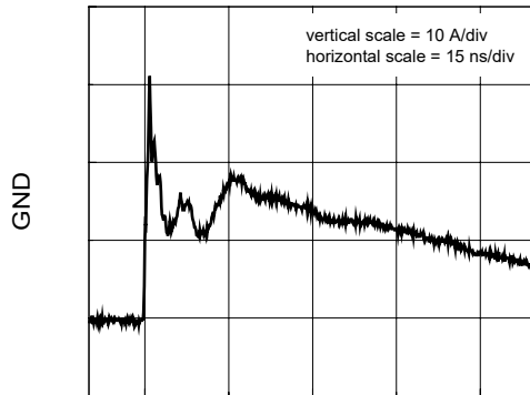
Figure 1: unclamped +8 kV ESD pulse waveform (IEC 61000-4-2 network)
