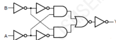
Figure 3. Logic diagram
