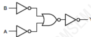
Figure 3. Logic diagram
