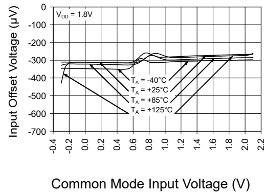
Figure 2: Input Offset Voltage vs. Common-Mode Input Voltage at V_{DD} = 1.8V .
