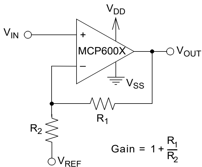
Noninverting Amplifier
