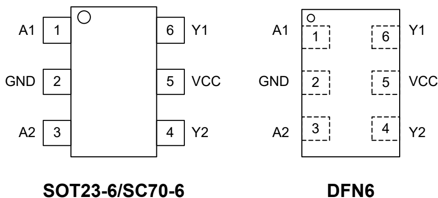
Figure1. Top View
