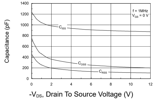
Figure 8: Capacitance Characteristics
