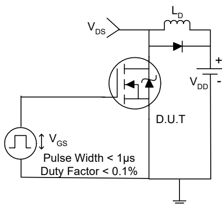
Figure 15: Gate Charge Test Circuit
