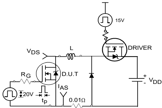
Figure 13a: Unclamped Inductive Test Circuit
