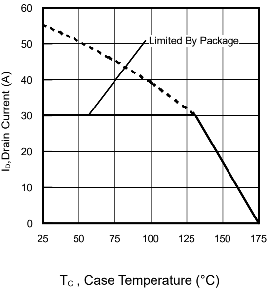
Figure 10: Maximum Drain Current vs. Case Temperature
