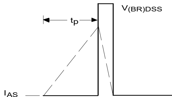
Figure 13b: Unclamped Inductive Waveforms
