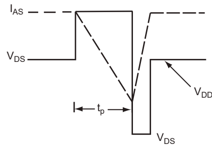
Figure 13b: Unclamped Inductive Waveforms
