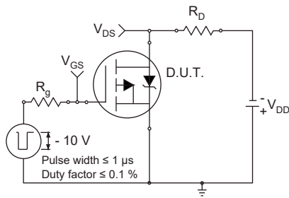
Figure 12a: Switching Time Test Circuit
