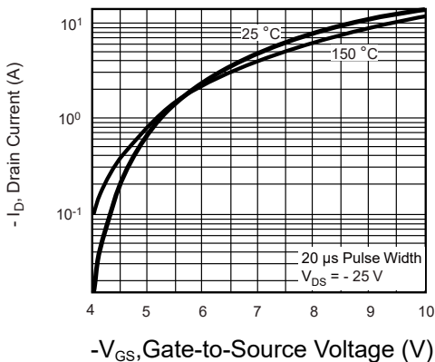
Figure 5: Typical Transfer Characteristics
