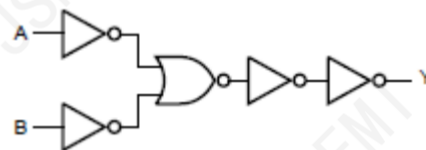
Figure 3. Logic diagram
