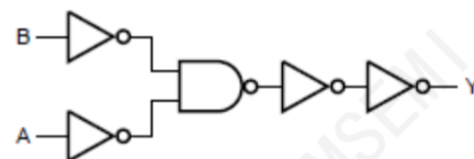
Figure 3. Logic diagram
