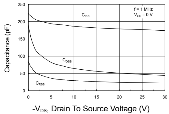
Figure 8: Capacitance Characteristics
