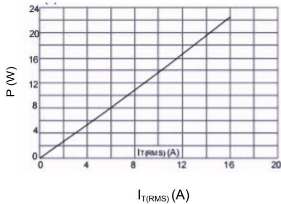
Figure 1: Maximum power dissipation versus RMS on-state current
