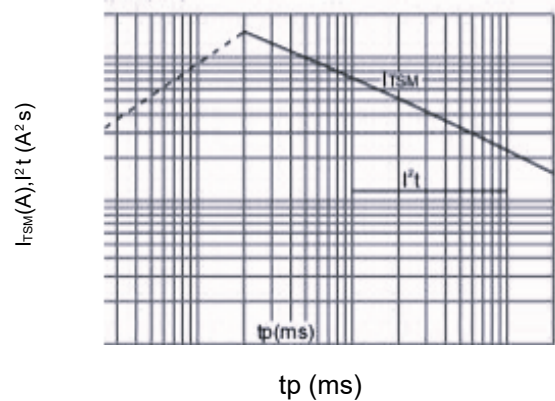
Figure 5: Sinusoidal pulse with width t_p < 20\text{ms} value of I^2t ( dIdt < 50\text{A}\mu\text{s} )
