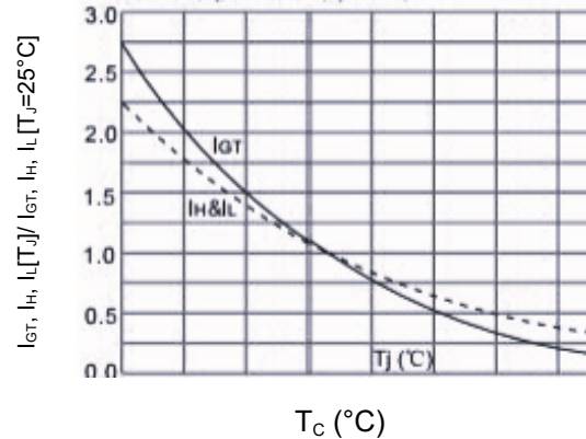
Figure 6: Holding current and latching current versus junction temperature
