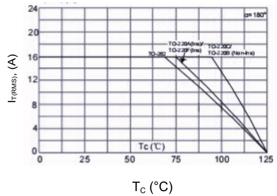
Figure 2: RMS on-state current versus case temperature
