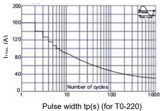
Figure 3: Surge peak on-state current versus number of cycles
