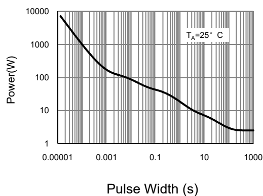
Figure 15: Single Pulse Power Rating Junction-to-Case (Note F)
