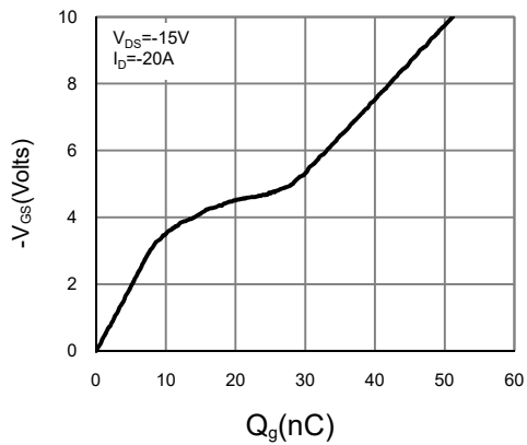
Figure 7: Gate-Charge Characteristics
