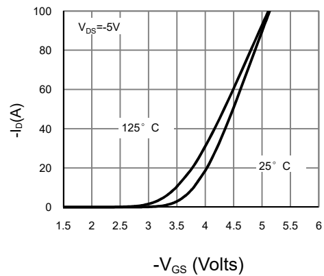
Figure 2: Transfer Characteristics (Note E)
