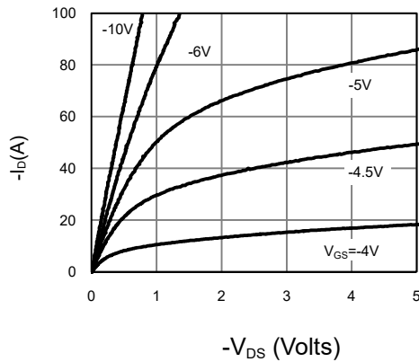
Fig 1: On-Region Characteristics (Note E)
