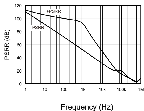
Figure 5: Power-Supply Rejection Ratio vs Frequency
