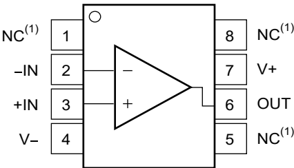
SOP-8
