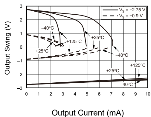
Figure 6: Output Voltage Swing vs Output Current
