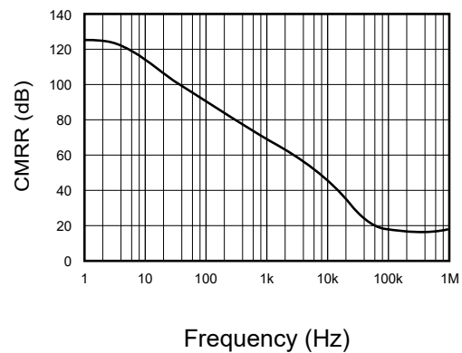
Figure 4: Common-Mode Rejection Ratio vs Frequency
