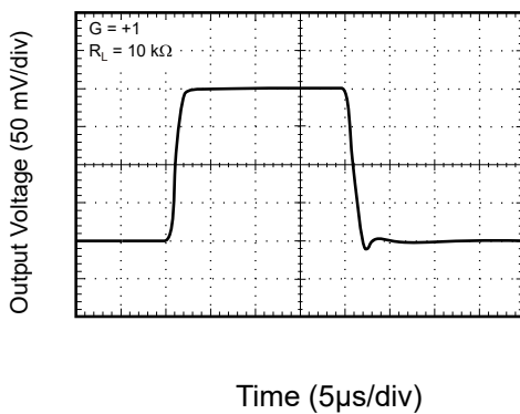
Figure 11: Small-Signal Step Response
