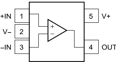
SC70-5
