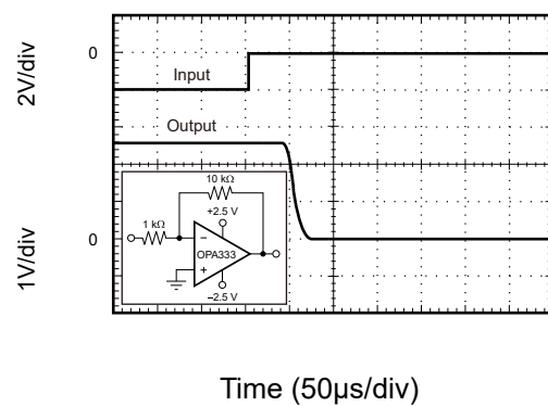
Figure 12: Positive Overvoltage Recovery
