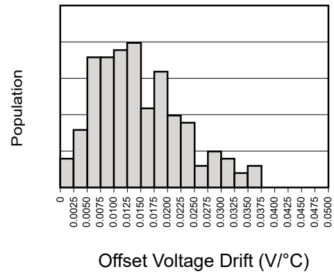
Figure 2: Offset Voltage Drift Production Distribution
