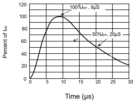
Figure 3: Pulse Waveform-8/20 \mu\text{s}
