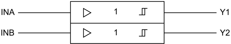
Figure2. Logic Symbol
