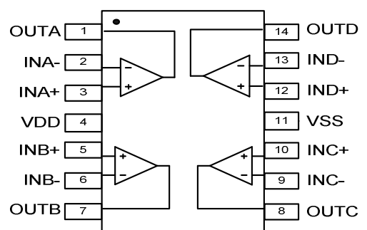
SOP-14 TSSOP-14
