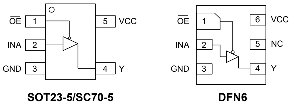
Figure1. Pinouts (Top View)
