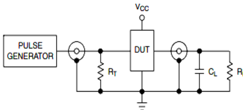
Figure4. Test Circuit
