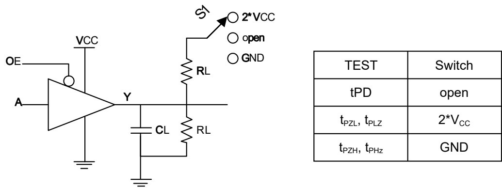
Figure5. Output enable/disable Time Test Circuit
