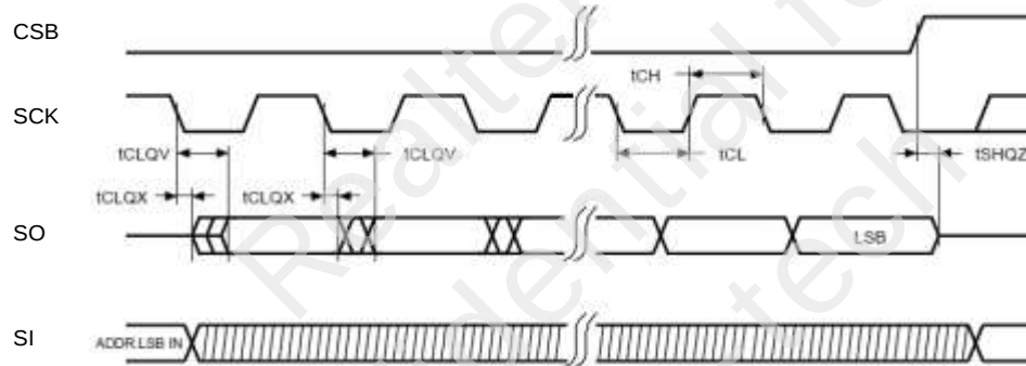
Figure 8. SPI Flash Interface Timing
