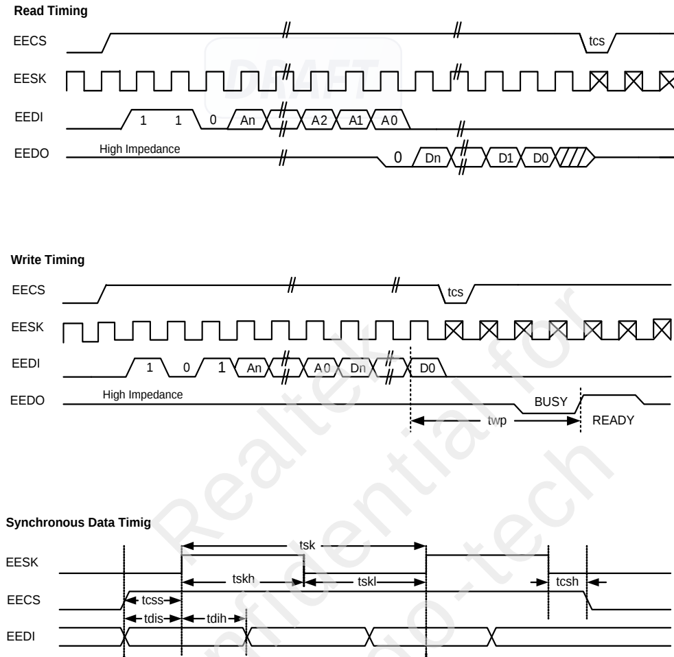
Figure 2. 3-Wire EEPROM Interface Timing
