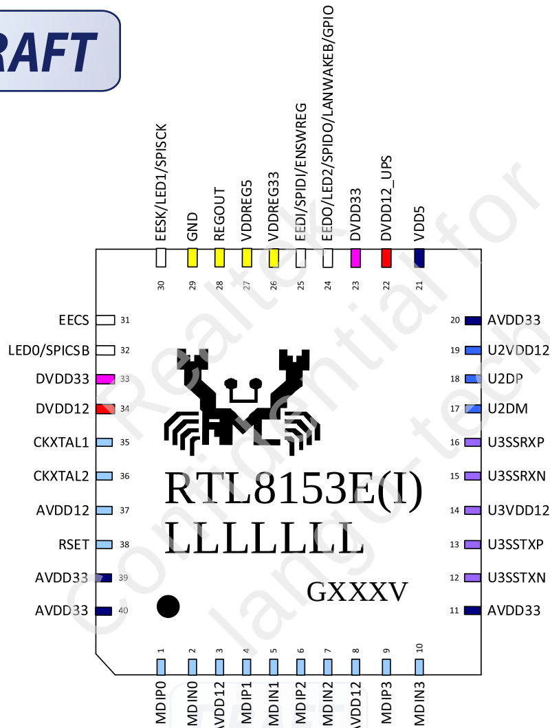
Figure 1. Pin Assignments
