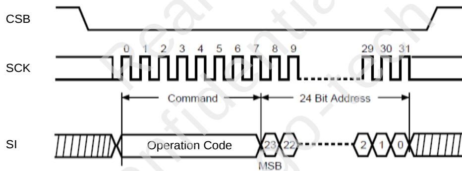
Figure 6. Sector/Block Erase Command Sequence
