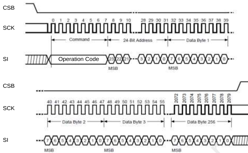
Figure 5. Page Program Command Sequence
