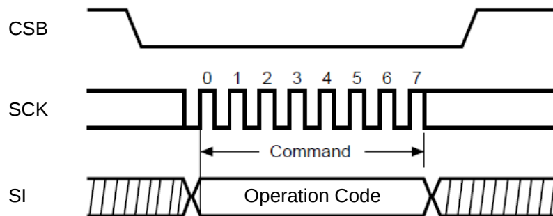
Figure 7. Chip Erase Command Sequence
