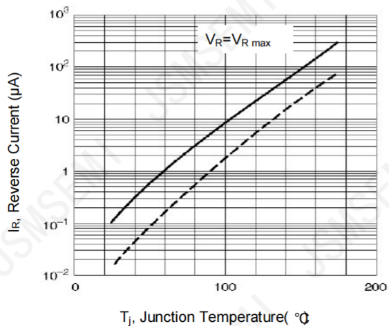
Fig 5. Reverse Characteristics
