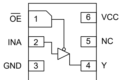
DFN6
