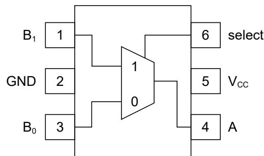
SC70-6/SOT23-6
