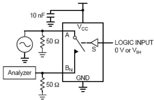
Figure 4: Turning off
