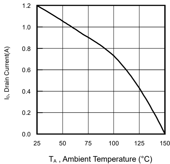
Fig 13. Maximum Drain Current vs. Ambient Temperature
