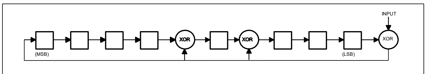
Figure 9. CRC Generator
