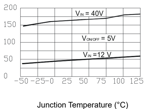
Figure 4: Standby Quiescent Current
