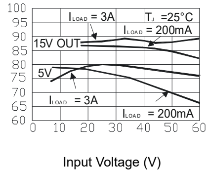
Figure 8: Efficiency
