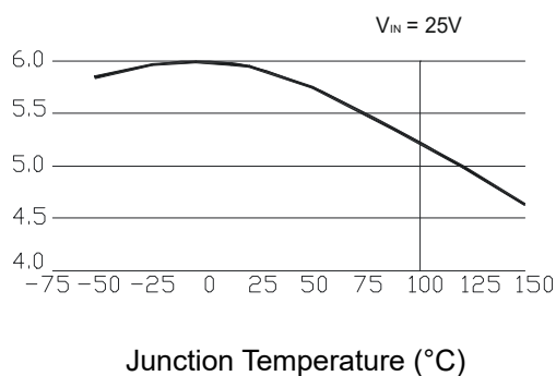
Figure 6: Current Limit
