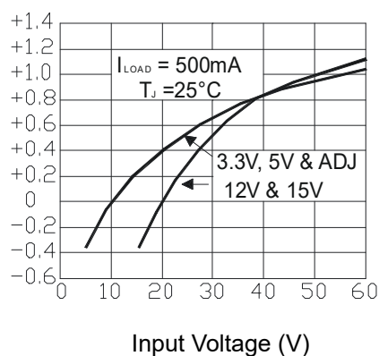
Figure 2: Line Regulation
