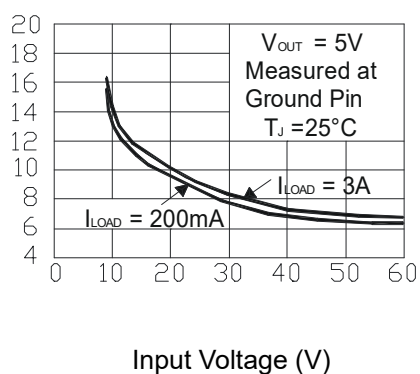
Figure 5: Quiescent Current
