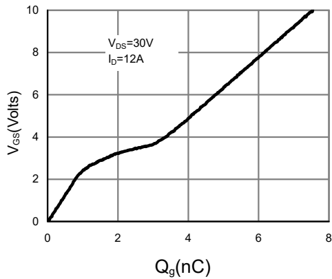
Figure 7: Gate-Charge Characteristics
