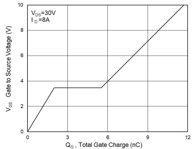
Fig.4 Gate-Charge Characteristics
