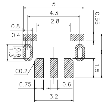
PCB. 焊接图 PCB. WELDING DRAWING
