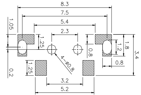
PCB. 焊接图 PCB. WELDING DRAWING
