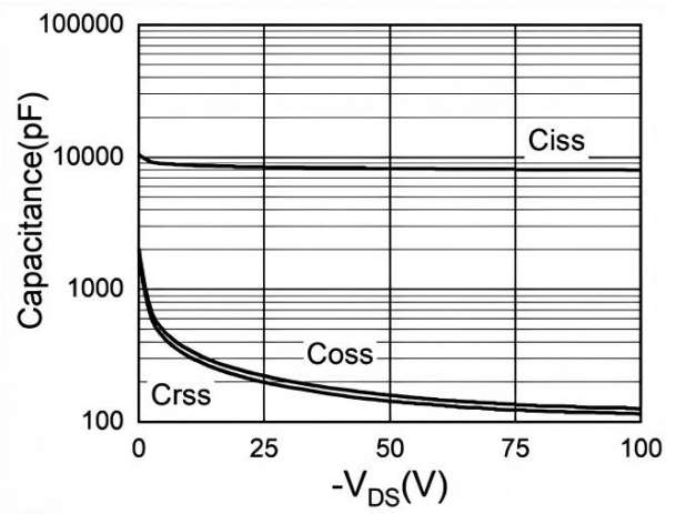
Figure 8. Capacitance
