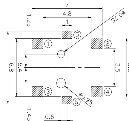
(PCB焊接参考图) PCB. WELDING DRAWING
