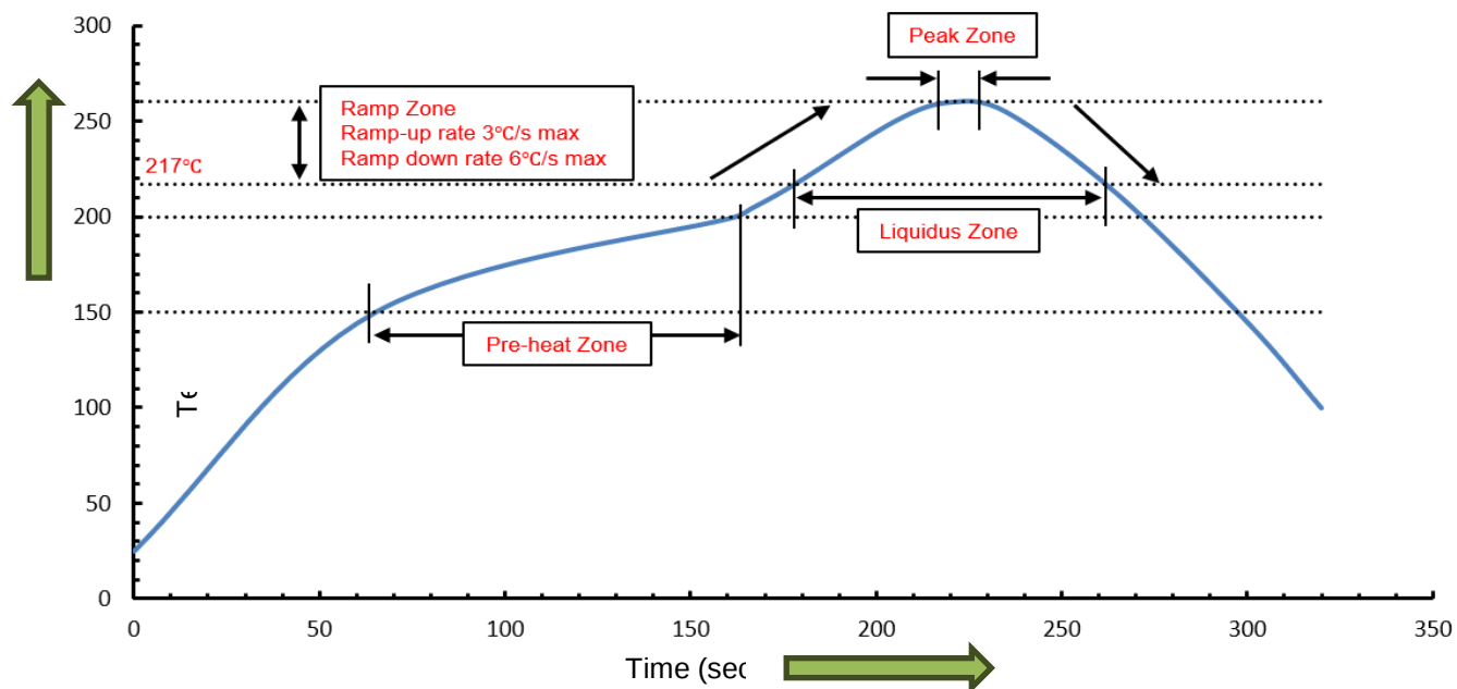
Reflow Profile
