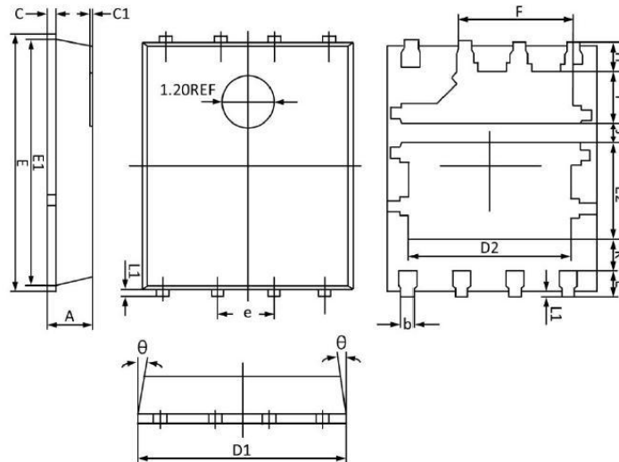
PRPAK5*6 Dual Asymmetric Package Outline
