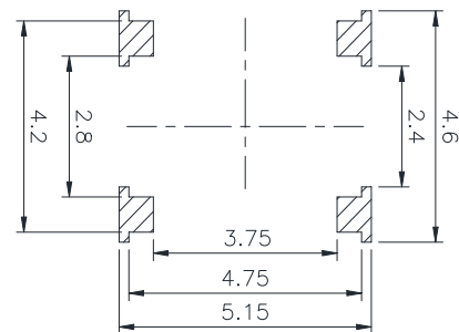
PCB. 焊接图 PCB. WELDING DRAWING
