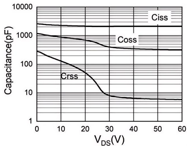
Fig.8 Capacitance
